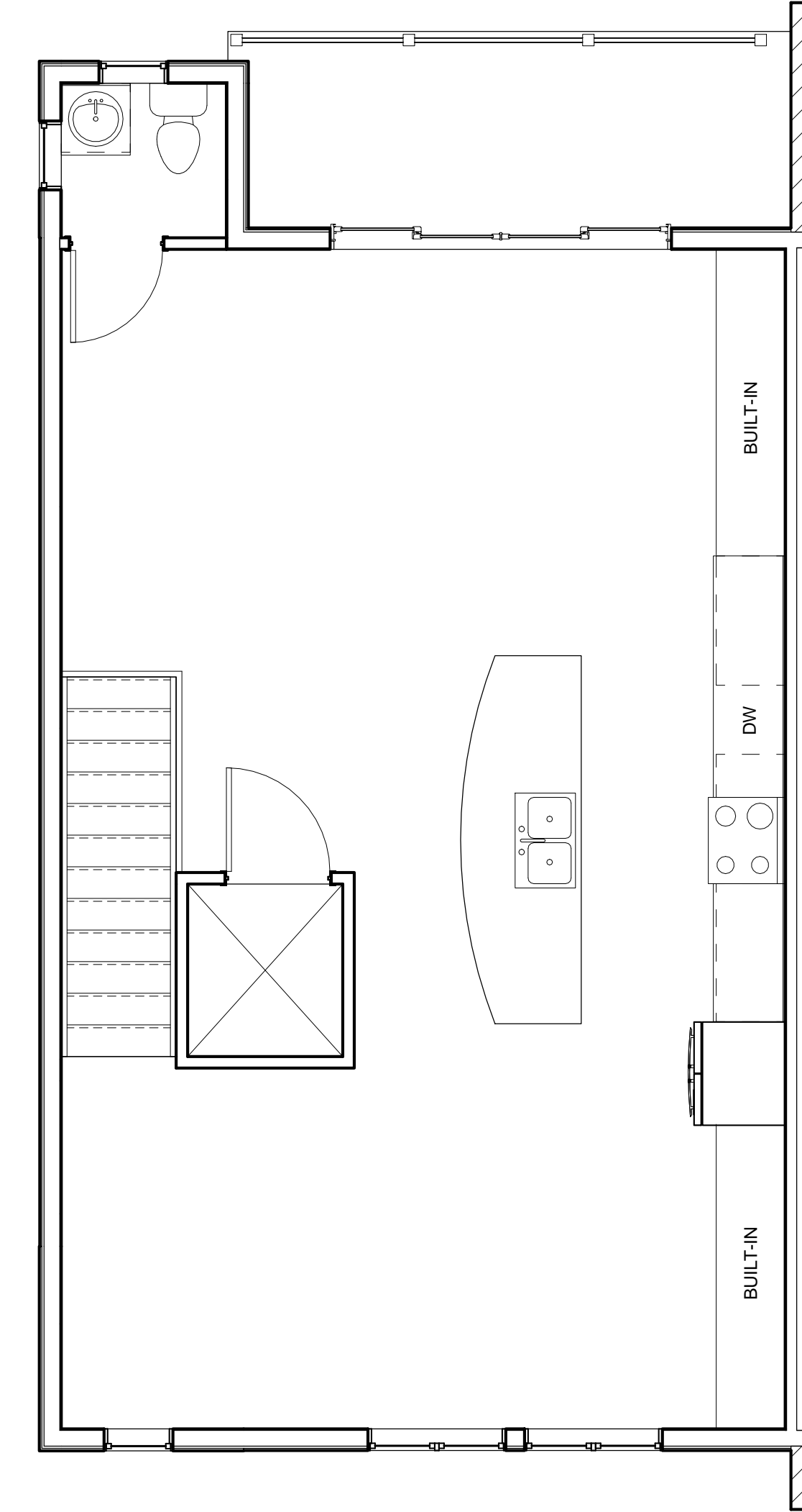
③ Small Unit Level 3 1/4" = 1'-0"
